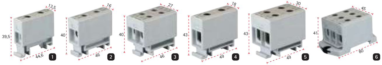
Maße in mm | Dimensions in mm | Gabarit en mm
