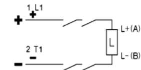
Connection diagram 2-pole: don't use attached jumper
