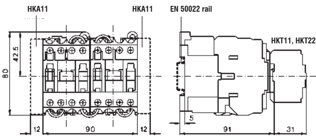
K3PV-30A00, K3PV-60A00
