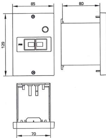
Moulded Front Plate MU25-C55
