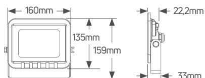
Floodlight 30W Black
