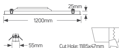
LED Line Recessed 40W 1.2m
