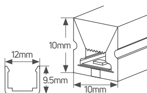
Neon LED strip 24V 10x10mm
