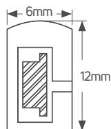
Neon LED strip 24V 6x12mm
