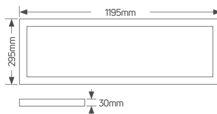
Panel Lithos 120x30 UGR<19
