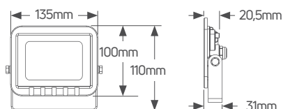
Floodlight 20W Black
