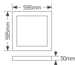
Panel Lithos 60x60 UGR<19
