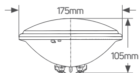
LED PAR56 18W
