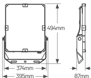
Himor 200W
