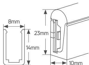
Neon LED strip 24V 10x23mm
