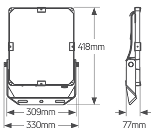
Himor 100W
