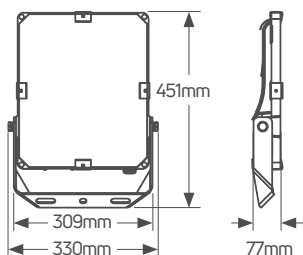
Himor 150W
