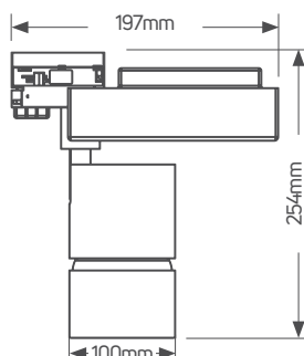
LED Track light 30W
