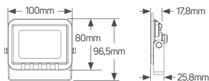
Floodlight 10W Black
