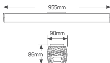
LED Linear Highbay 150W
