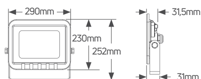
Floodlight 100W Black
