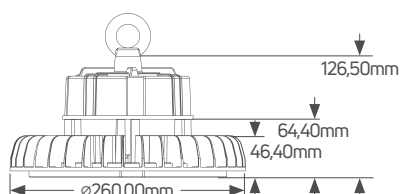
Highbay Premium 100W
