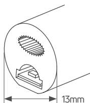
Neon LED strip 24V ø13mm
