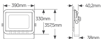
Floodlight 300W Black
