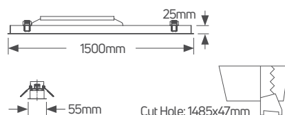
LED Line Recessed 50W 1.5m
