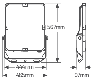
Himor 300W
