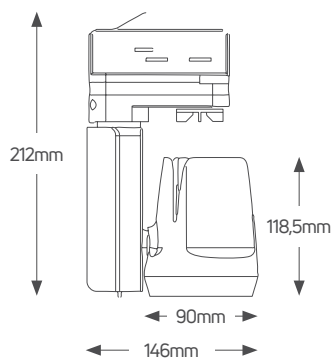
Track light 25W
