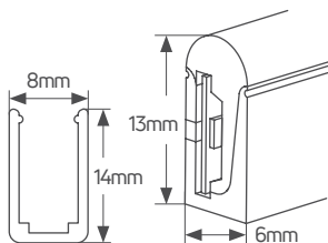
Neon LED strip 24V 6x13mm
