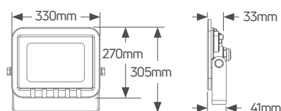
Floodlight 150W Black
