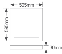
Panel Avra 60x60 UGR<19
