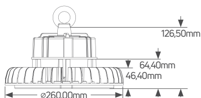
Highbay Premium 60W
