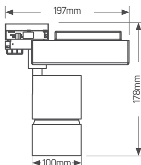
LED Track light 15W
