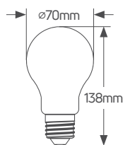
LED Bulb 12W, Sensor Day/Night
