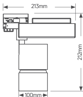
LED Track light 45W
