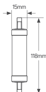
LED R7s 118mm 9W
