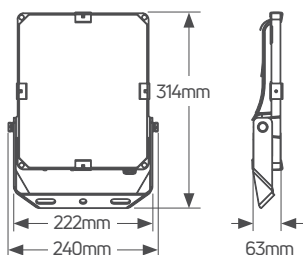
Himor 50W
