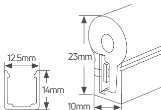
Neon LED strip 24V 10x23mm
