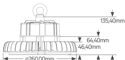
Highbay Premium 150W
