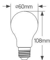
LED Bulb 9W, Sensor Day/Night
