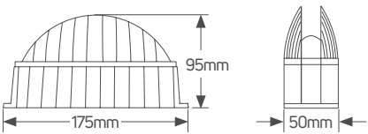
Window Light 8W
