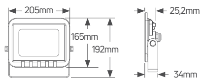
Floodlight 50W Black
