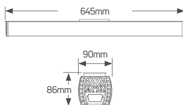
LED Linear Highbay 100W
