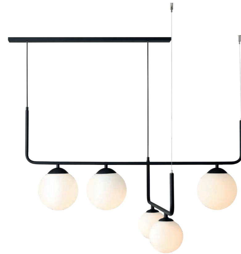
ARTEMIDA 5 BLACK 1060F1 | W108xH120xD78 | 3x E27 max.60W, 2x E 14 max.40W
